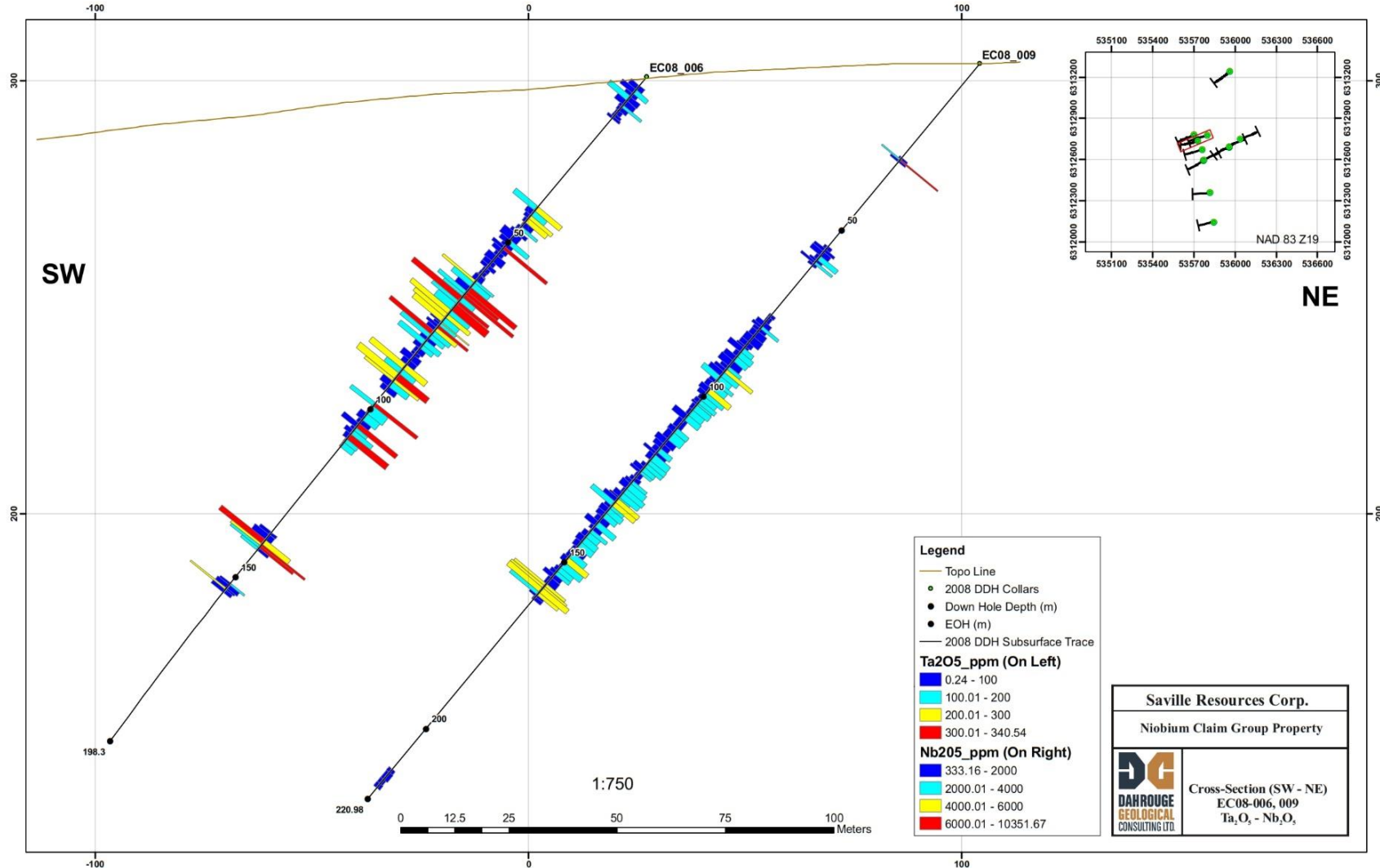
Figure 22: Cross-section downhole of Nb-Ta grade (EC08-006, and 009)
