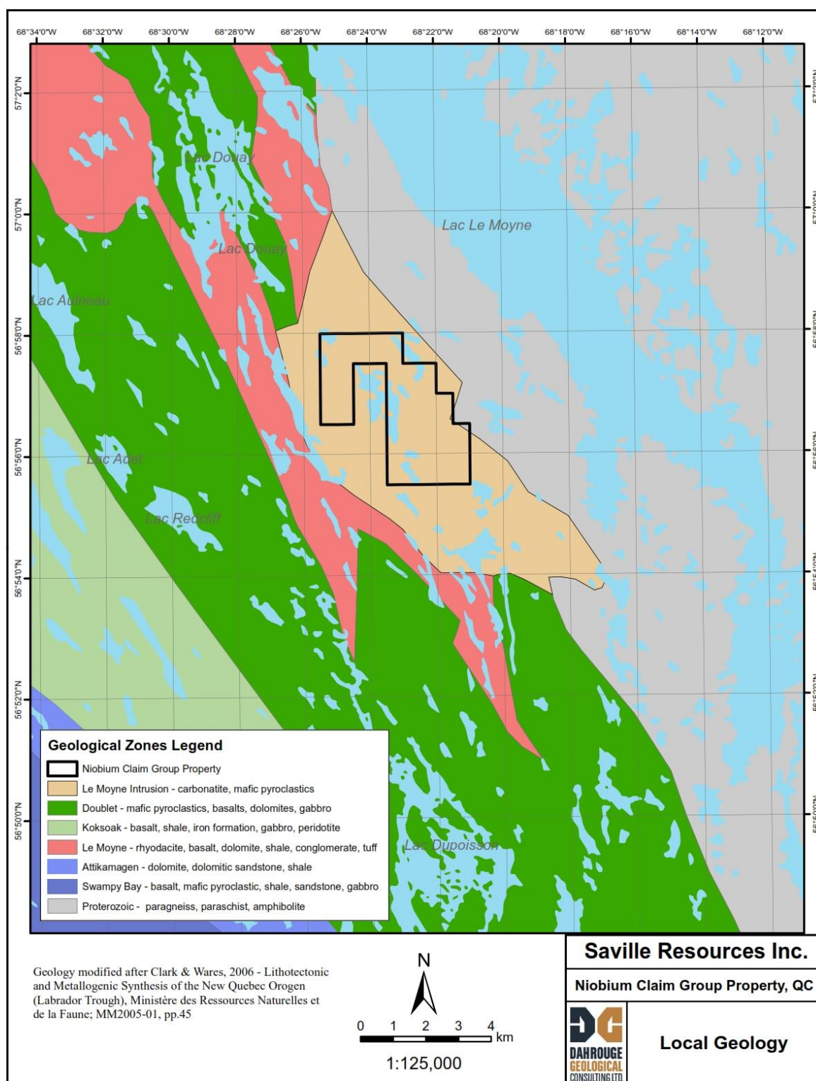
Figure 16: Local geology
